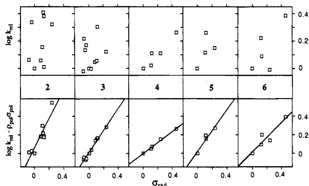
Figure 2. Semilogarithmic plots of the relative thermolysis rate constants ( k_{\text{rel}} ) for azoalkanes 2–6 , taken from the literature, 3c,9,10 versus the Creary \sigma_{\text{rad}} values. 6 The upper row contains the one-parameter plots without inclusion of polar contributions, and the lower row shows the two-parameter plots with polar contributions ( \rho_{\text{pol}}\sigma_{\text{pol}} ) included according to eq 6. The \rho_{\text{pol}} values were taken from Table 2 and the \sigma_{\text{pol}} values from ref 20. Note that the plots for azoalkane 3 do not contain the value for m\text{-OMe} , which might be in error (see footnote k in Table 2 and text). For correlation coefficients and slopes ( \rho_{\text{rad}} ), see Table 2.
