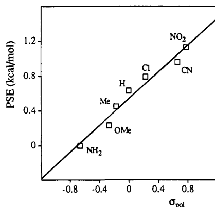
Figure 5. Plot of the calculated (AM1) ground state polar stabilization energies (PSE) for azocumene 2 relative to the alkane 8 for different para substituents X versus the Hammett \sigma_{\text{pol}} values. 20 Calculated data taken from Table 3 with \text{PSE} = [\Delta H_f(\text{azo-X}) - \Delta H_f(\text{azo-NH}_2)] - [\Delta H_f(\text{alkane-X}) - \Delta H_f(\text{alkane-NH}_2)] .
